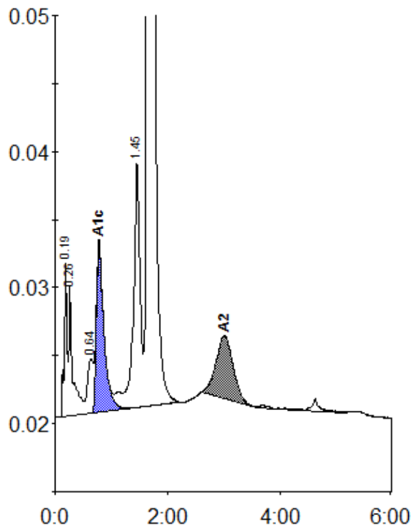
Peak table - ID: 10099342
