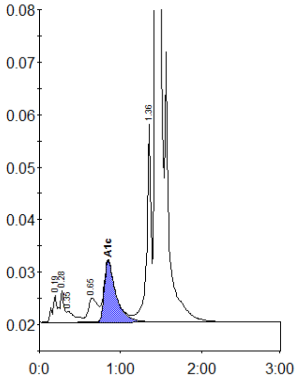
Peak table - ID: 10066101
