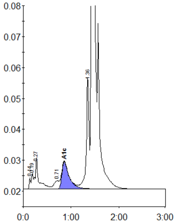
Peak table - ID: 10059932
