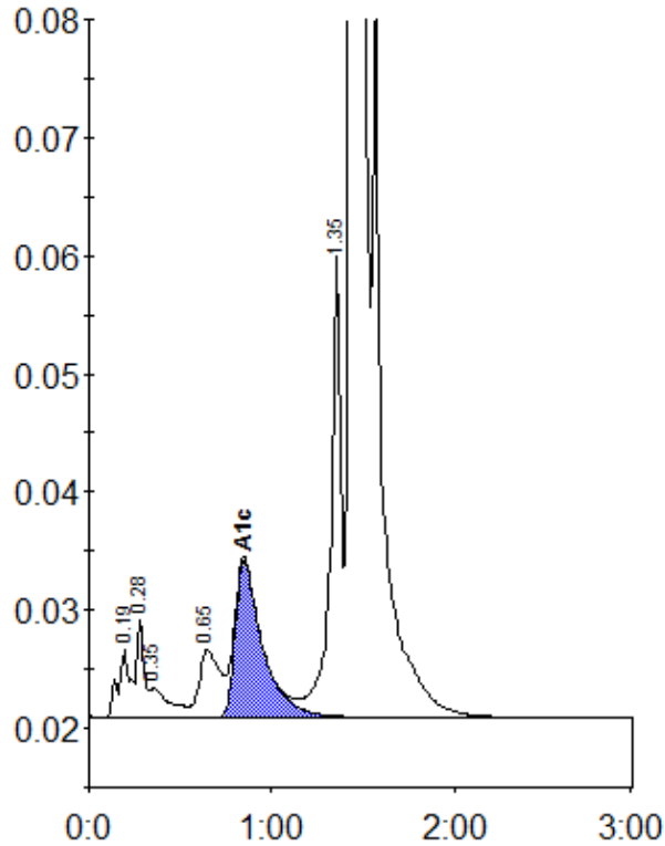
Peak table - ID: 10051778
