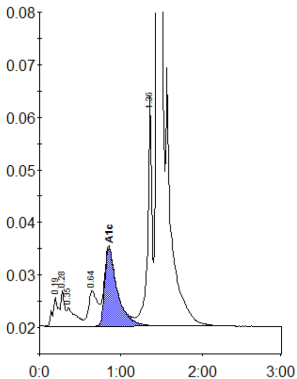
Peak table - ID: 10097946
