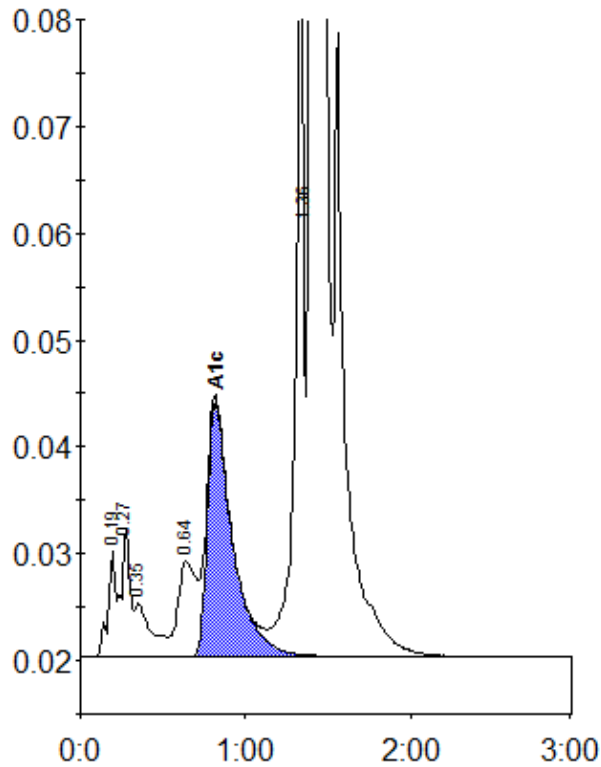
Peak table - ID: 10110558
