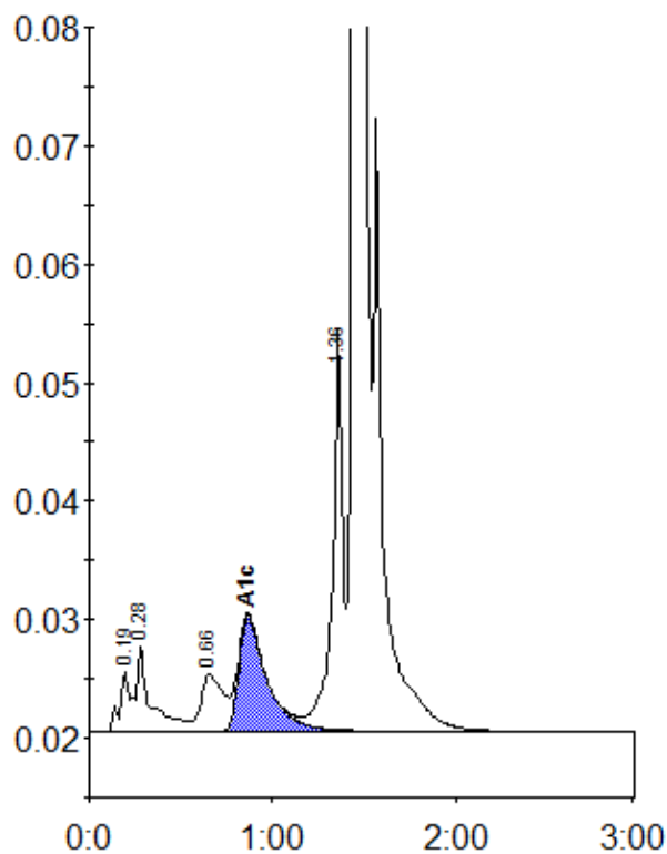
Peak table - ID: 10116846
