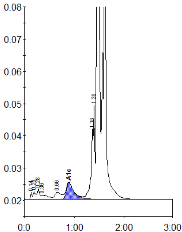
Peak table - ID: 10110866
