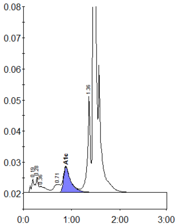
Peak table - ID: 10129421
