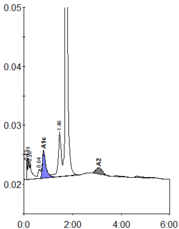
Peak table - ID: 0081497
