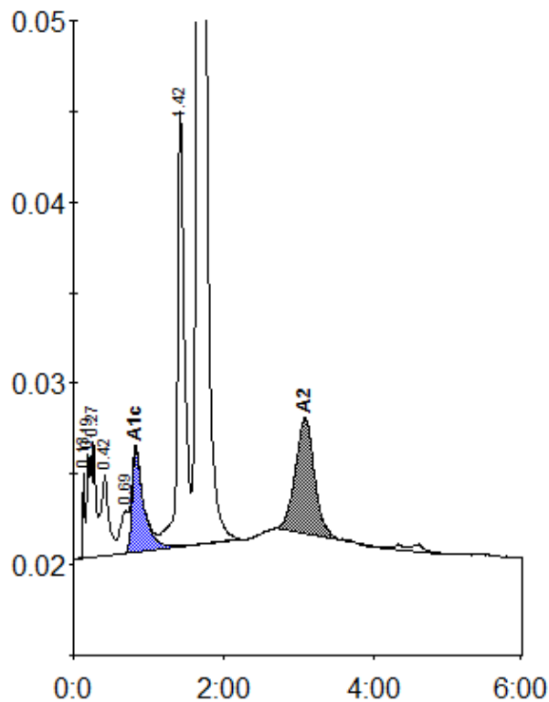
Peak table - ID: 10066907
