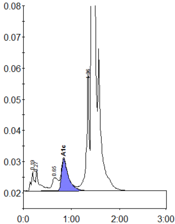
Peak table - ID: 10038961
