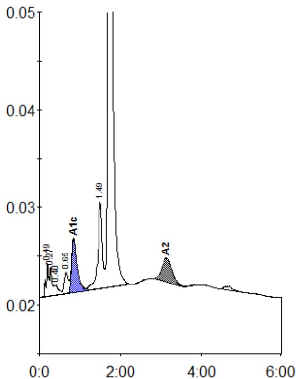
Peak table - ID: 10037027
