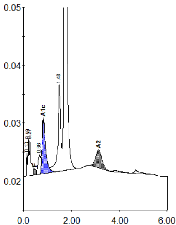
Peak table - ID: 10033898
