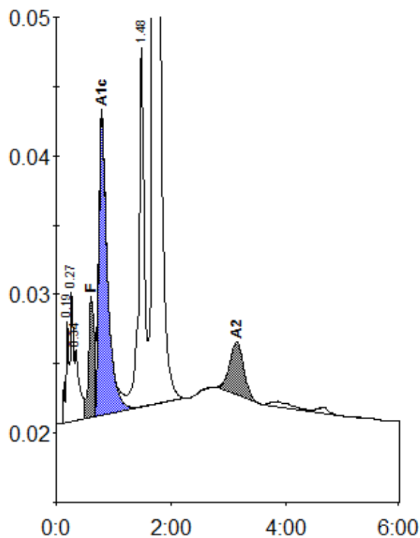
Peak table - ID: 10030930
