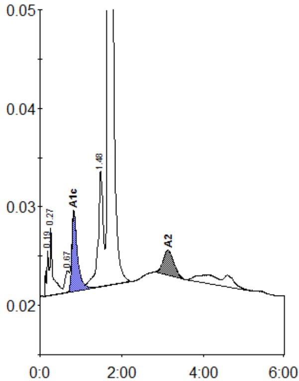
Peak table - ID: 10024879
