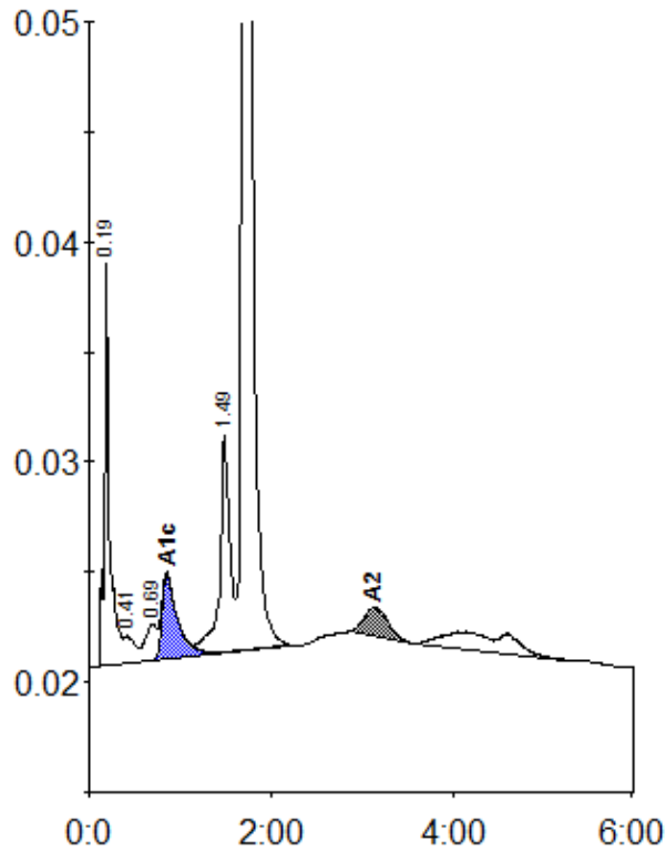
Peak table - ID: 10018819
