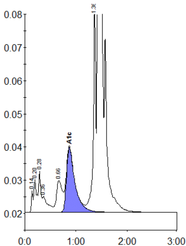
Peak table - ID: 10008811
