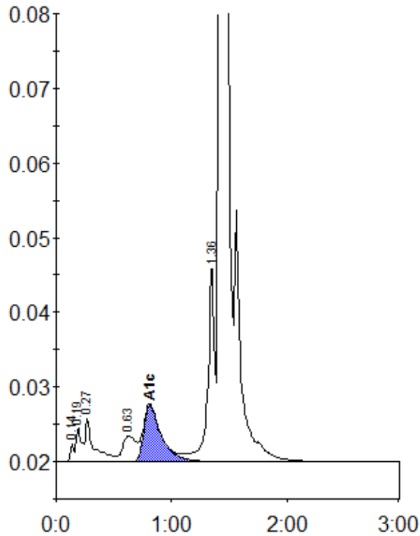
Peak table - ID: 10006408
