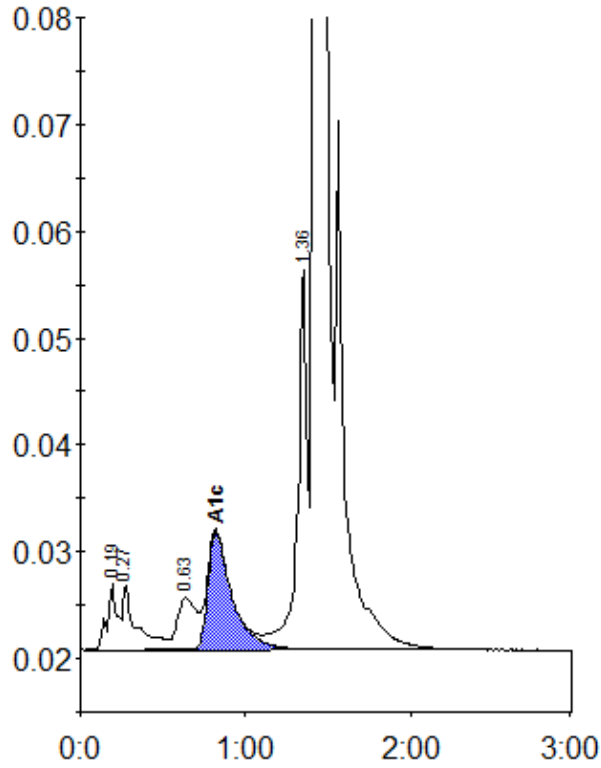
Peak table - ID: 10004699
