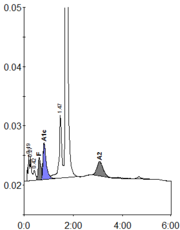
Peak table - ID: 10004469
