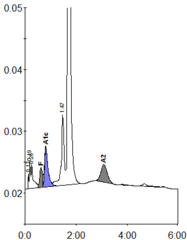
Peak table - ID: 10004468
