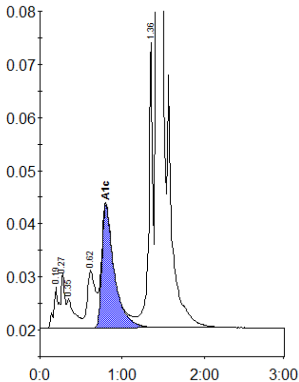
Peak table - ID: 10004068
