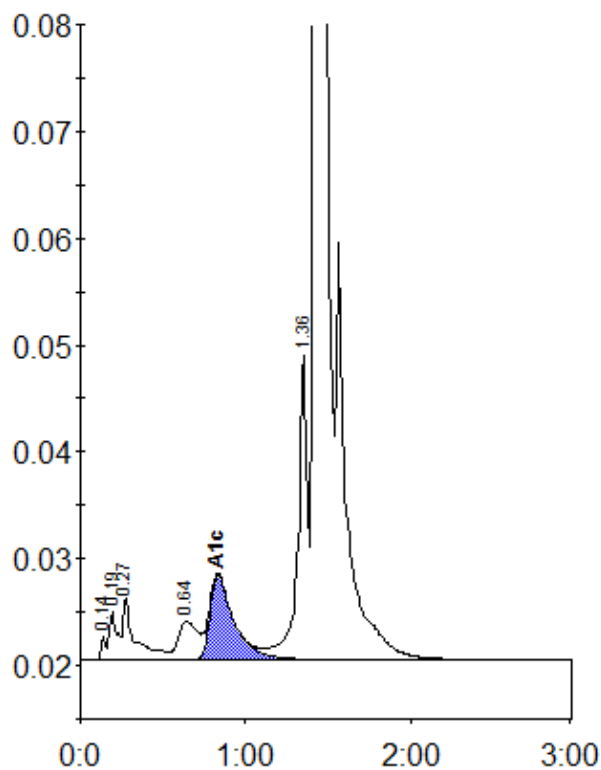
Peak table - ID: 10003307
