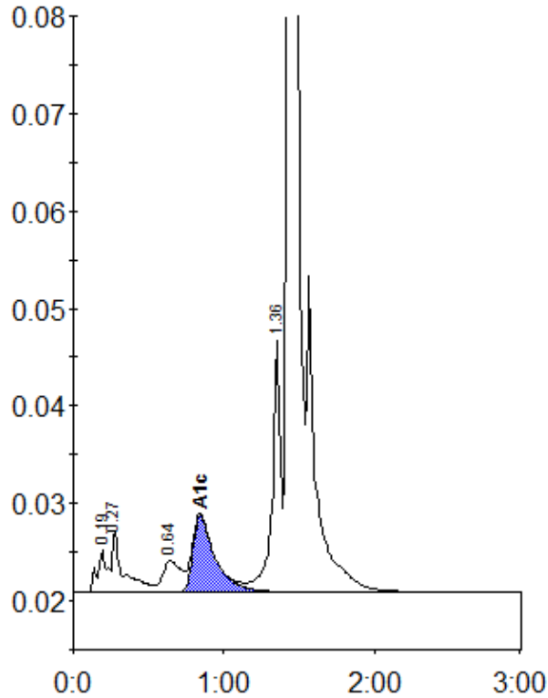
Peak table - ID: 10003054
