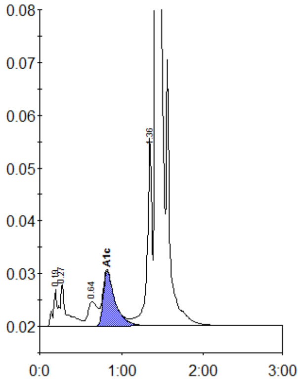
Peak table - ID: 10002149
