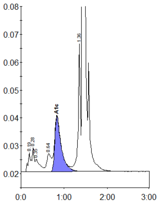
Peak table - ID: 10001220
