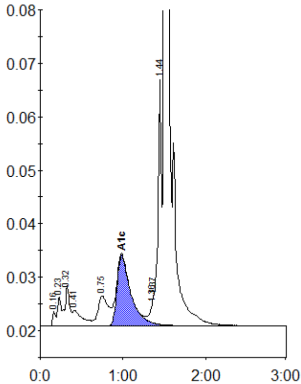
Peak table - ID: 10000885
