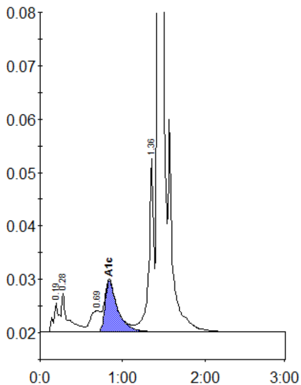
Peak table - ID: 10000463
