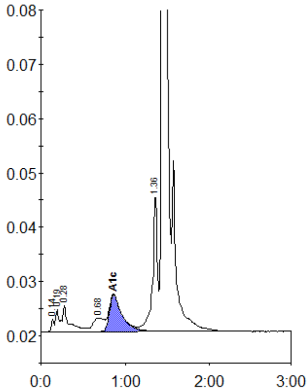
Peak table - ID: 01150088
