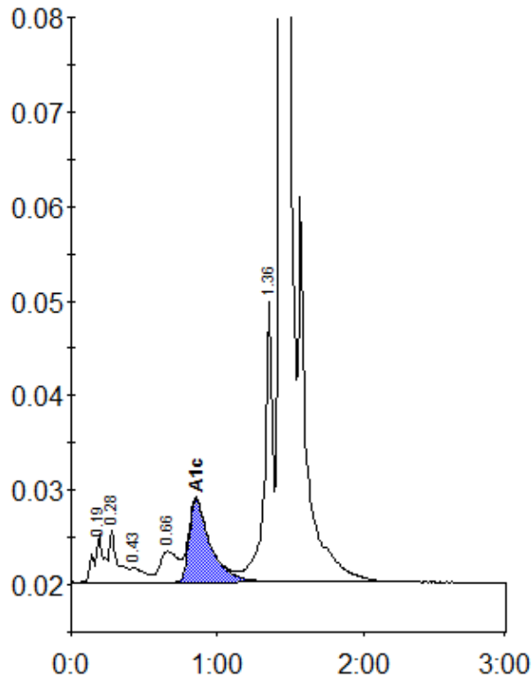
Peak table - ID: 01140070
