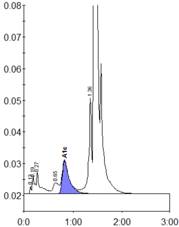
Peak table - ID: 01120062
