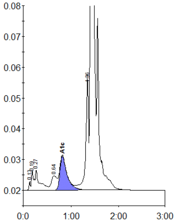
Peak table - ID: 01260026
