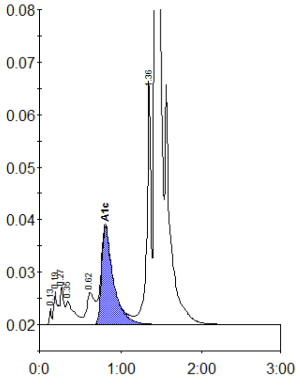
Peak table - ID: 01260144
