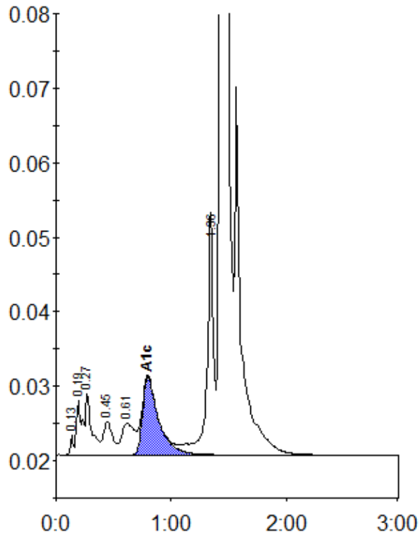
Peak table - ID: 01070014
