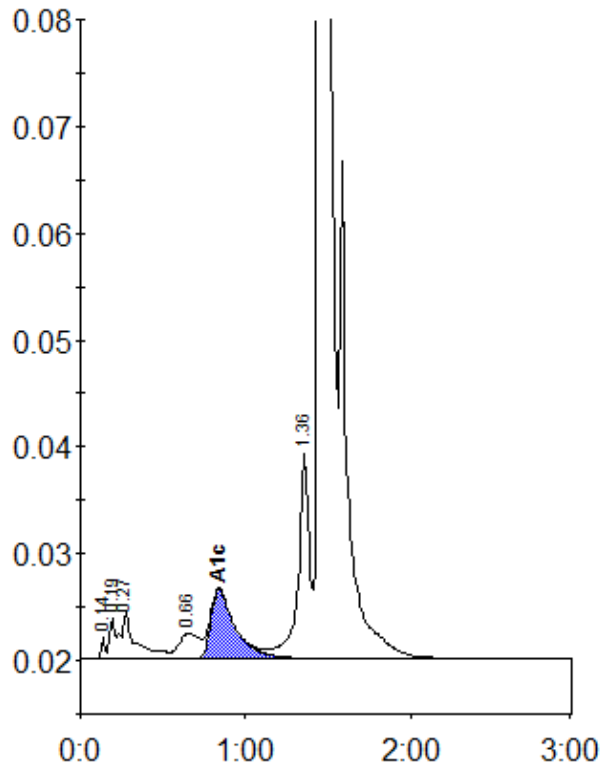
Peak table - ID: 01100055
