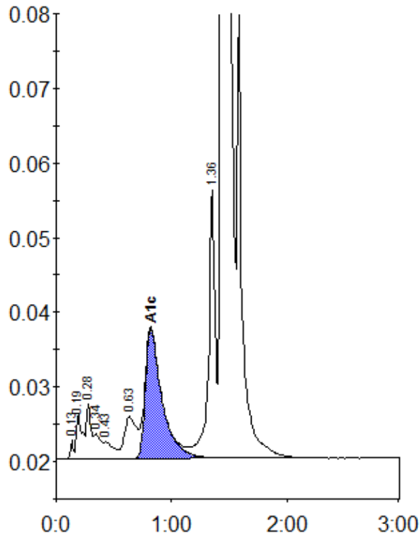
Peak table - ID: 01310023
