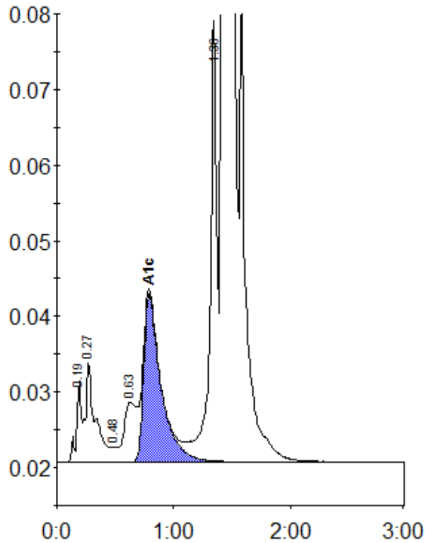
Peak table - ID: 01230027
